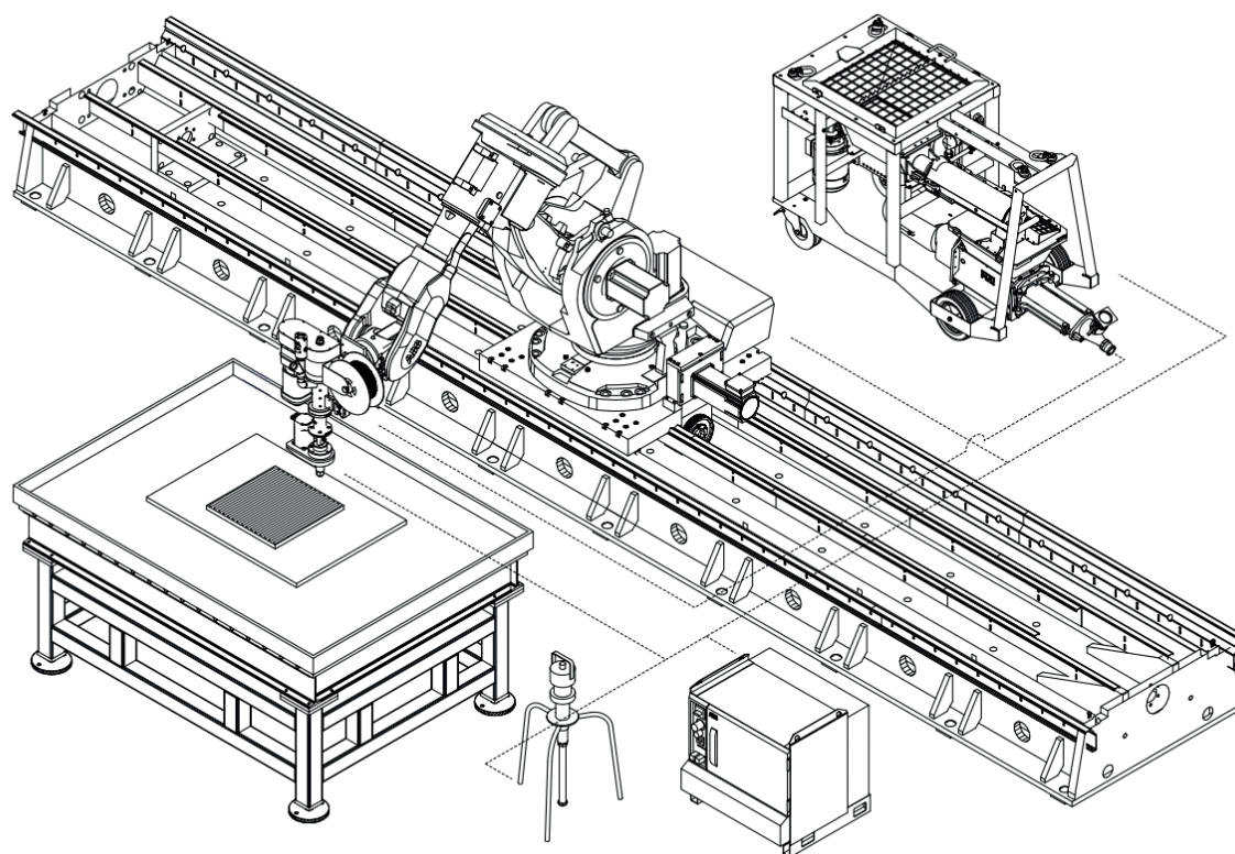
Diagram of a 3D printing production plant
